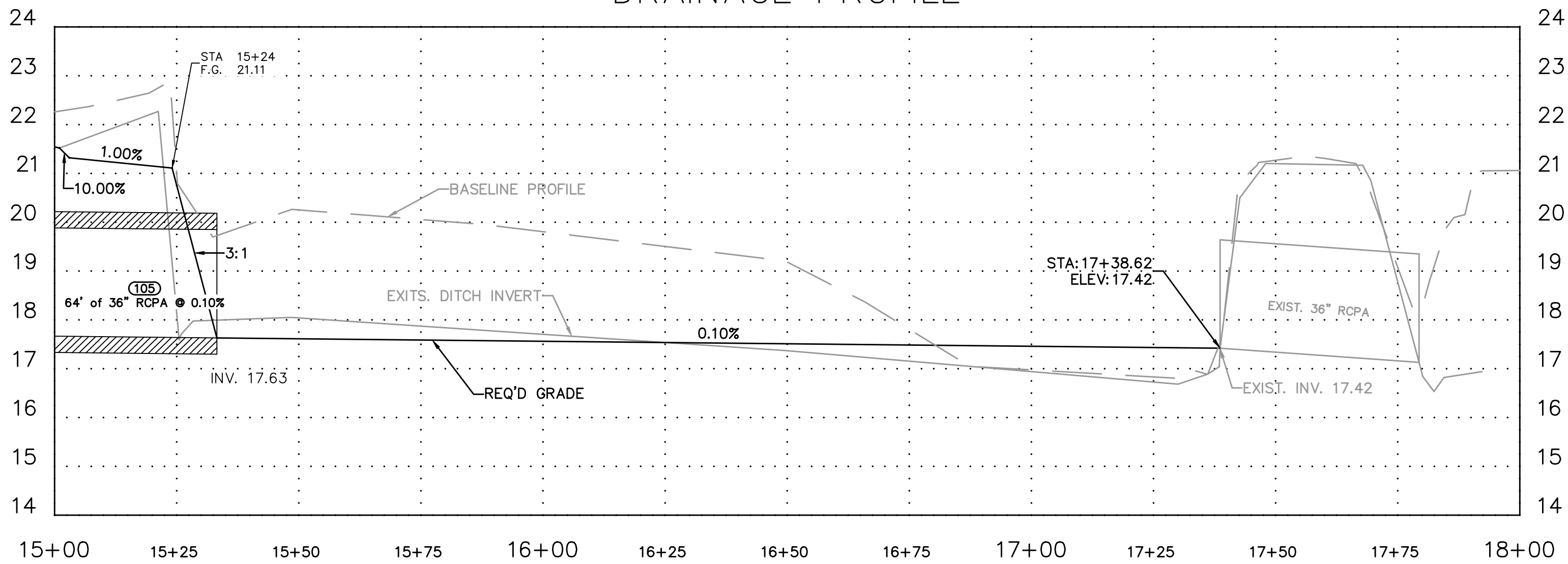
DRAINAGE PROFILE
